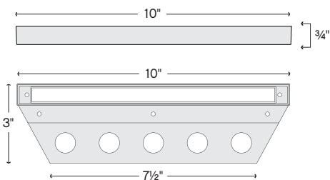
15448 TT NUVI™ LARGE DECK SCONCE 10" W, 3/4" H, 3" Dv 2 1/8" BRACKET DEPTH
