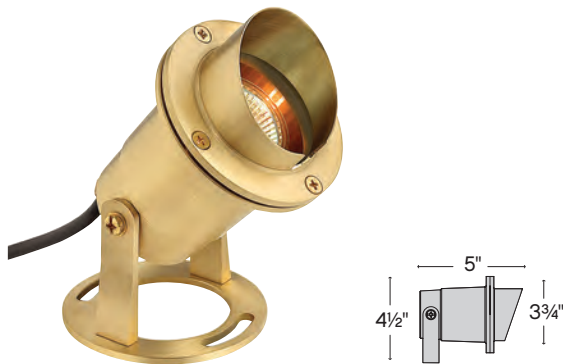
1539 BS MR16 BRASS SUBMERSIBLE POND LIGHT 3 3/4" DIA. SHROUD 5" W, 4 1/2" H
