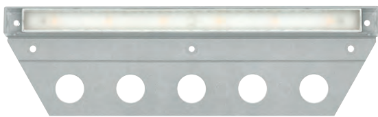
15448 TT NUVI™ LARGE DECK SCONCE 10" W, 3/4" H, 3" Dv 2 1/8" BRACKET DEPTH
