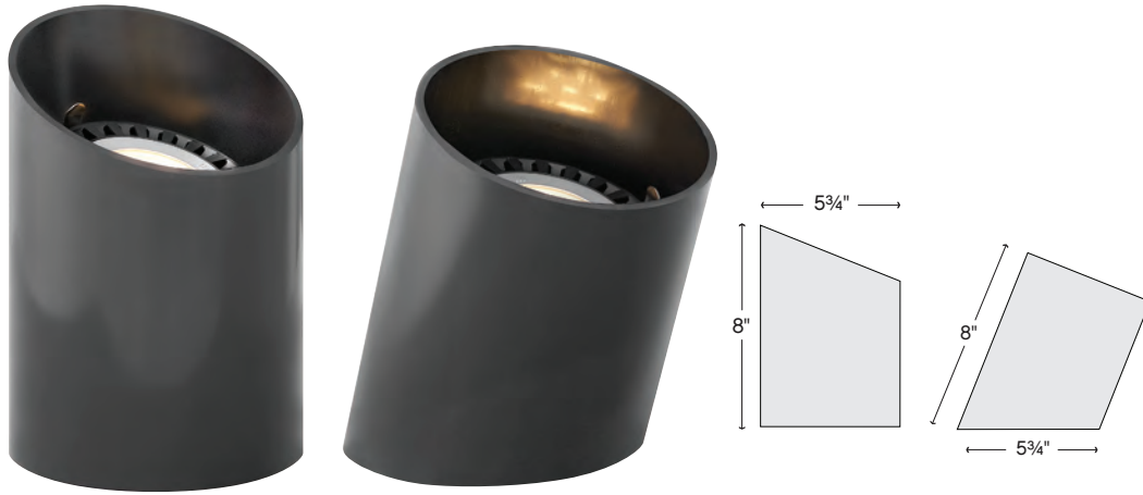
1598 BK REVERSIBLE PAR36 WELL LIGHT 5 3/4" DIA., 8" H
