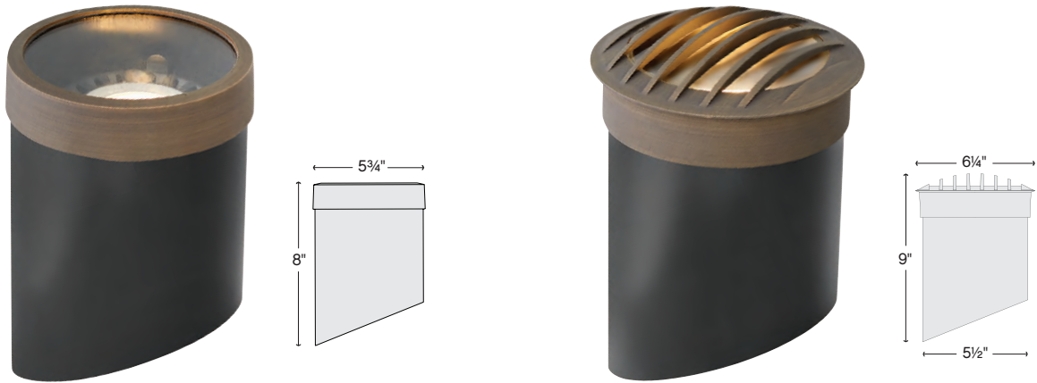
1598 MZ-FT HARDY ISLAND™ FLAT TOP PAR36 WELL LIGHT 5 3/4" DIA., 8" H
